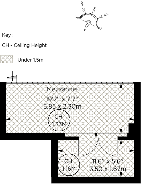
MEZZANINE
